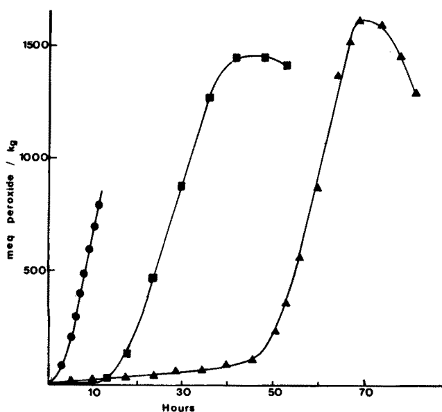
FIG. 1. Oxidation of jojoba wax by air under accelerated conditions (98 C). \blacktriangle , Crude wax; \bullet , stripped wax; \blacksquare , bleached wax.
